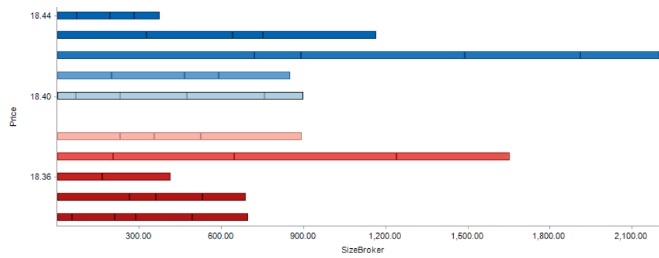
Figure 4-43. A horizontal numeric stacked needle graph.
