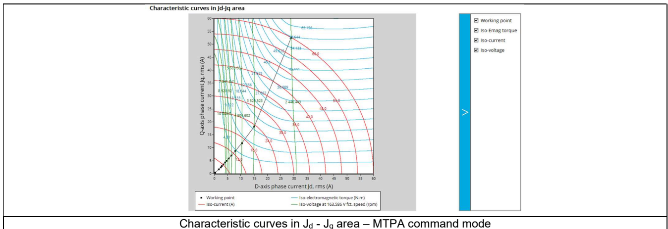
Characteristic curves in J_d - J_q area – MTPA command mode
