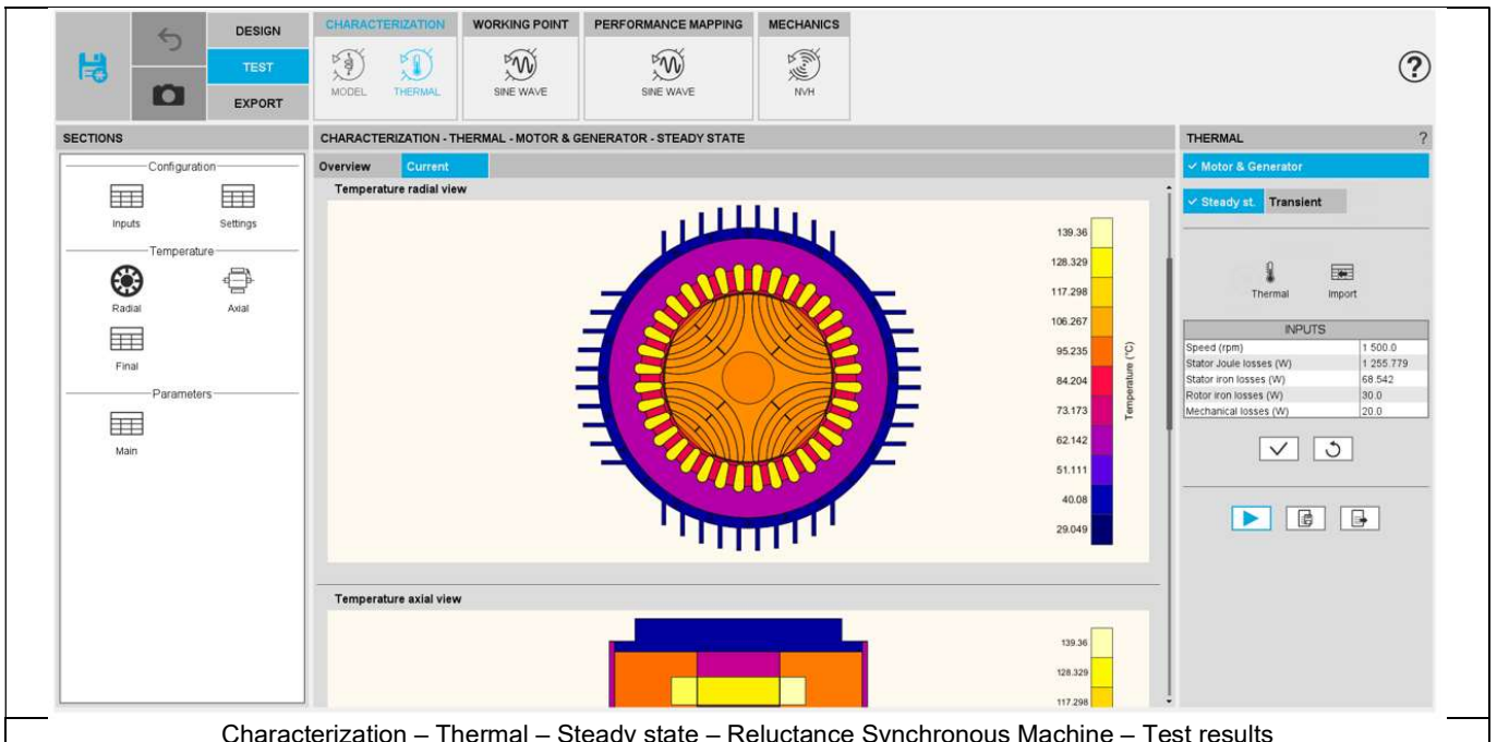
Characterization – Thermal – Steady state – Reluctance Synchronous Machine – Test results
