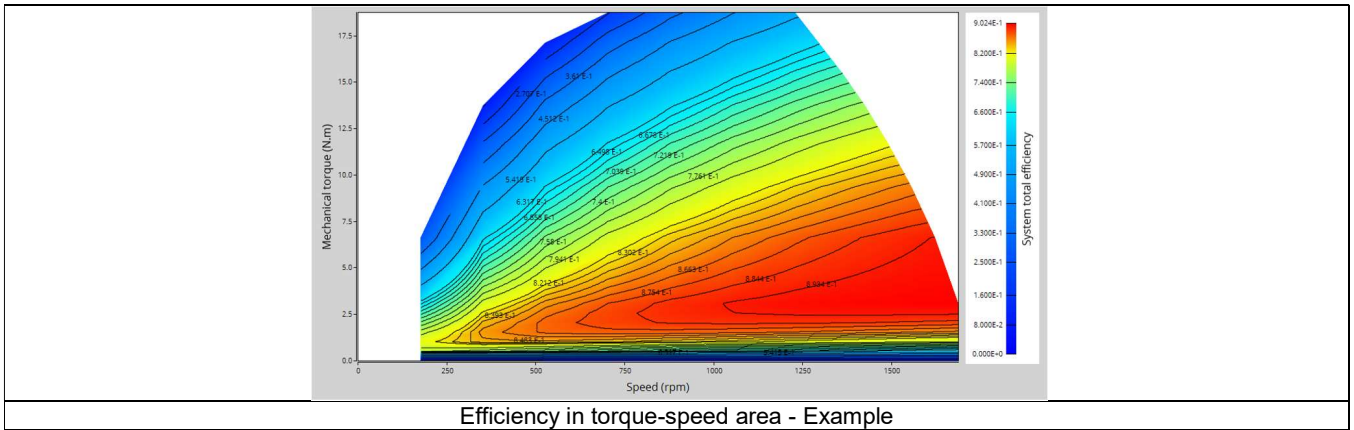
Efficiency in torque-speed area - Example
