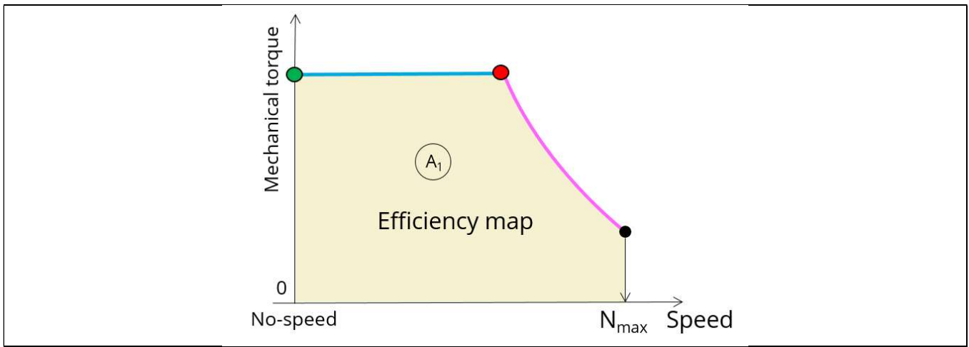
MTPA command modes – Efficiency map computation process
