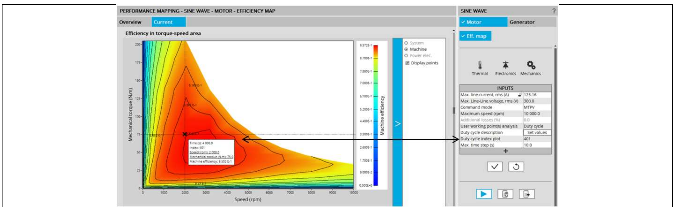
Selection of one working point of the driving cycle – Duty cycle index plot All the maps are updated considering the physical properties resulting from this working point
