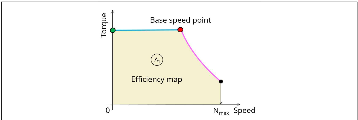
MTPA command modes – Efficiency map computation process
