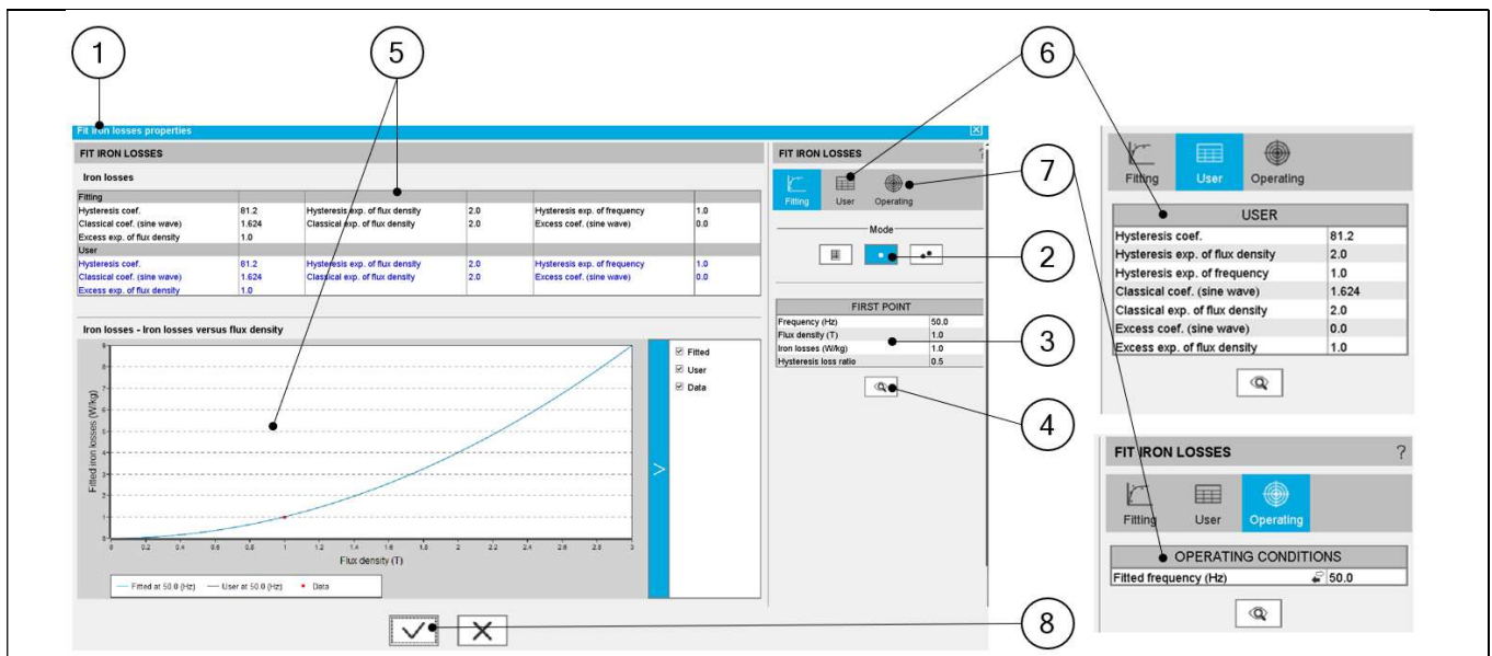
Definition of iron loss coefficients – from one measurement point
