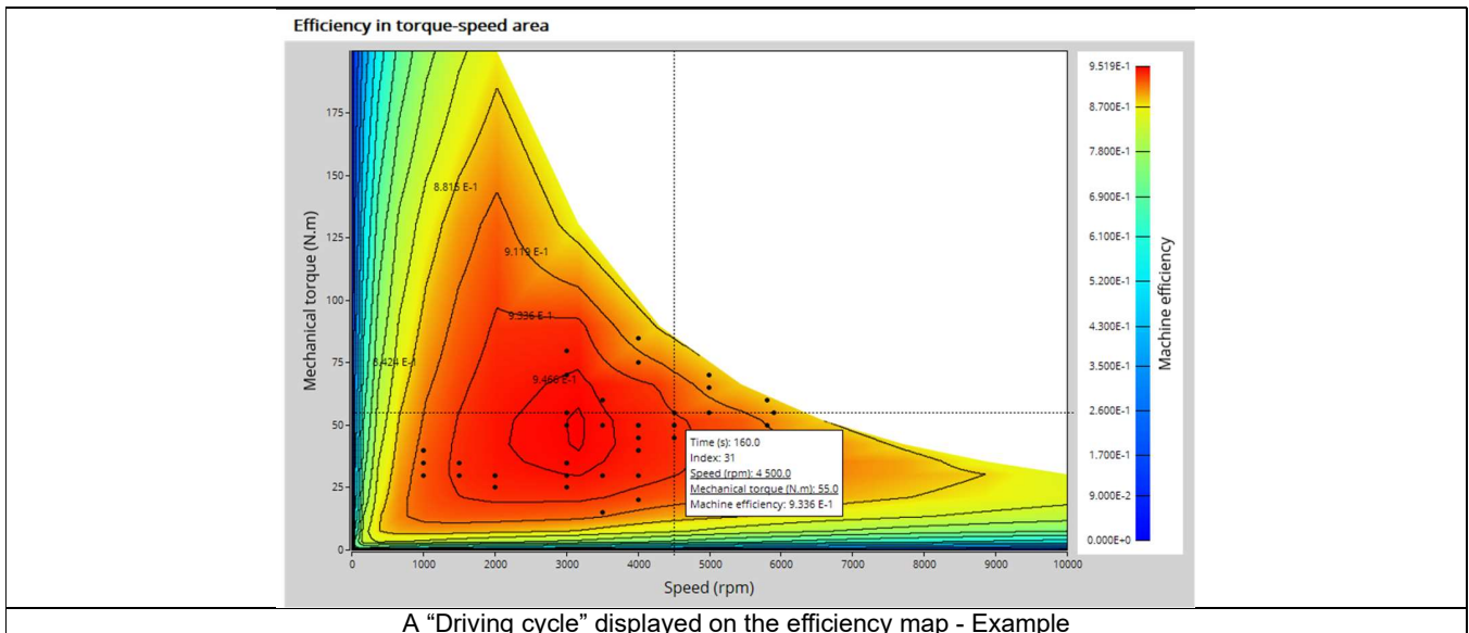
A "Driving cycle" displayed on the efficiency map - Example
