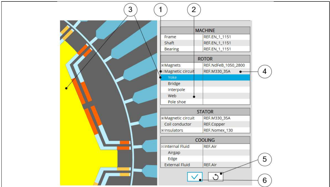
Assign materials to the rotor magnetic circuit
