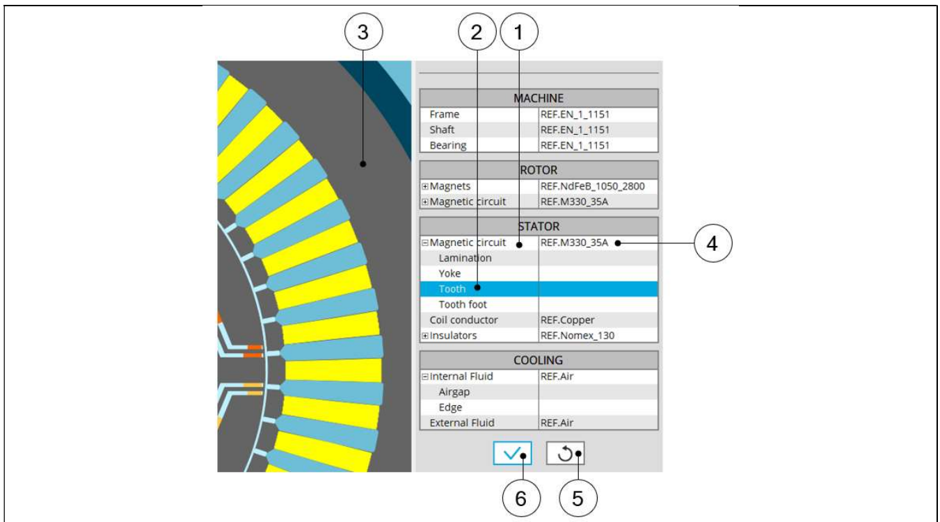
Assign materials to the stator magnetic circuit
