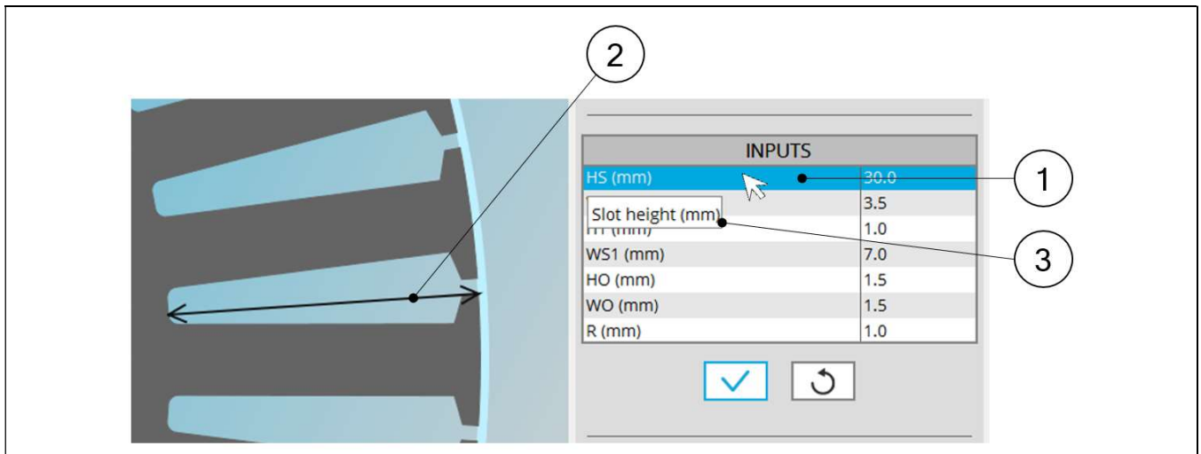
Inputs / Outputs stator slot
