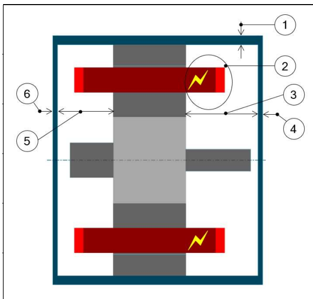
User input parameters to define frame dimensions in the axial view
