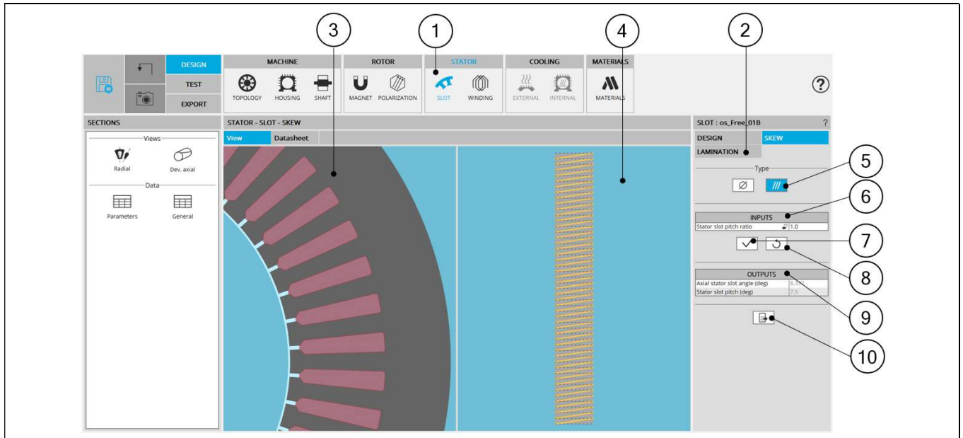
SLOT – SKEW design area
