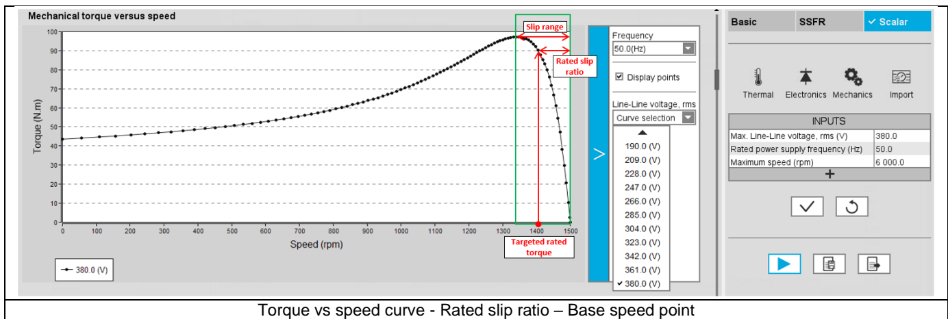
Torque vs speed curve - Rated slip ratio – Base speed point
