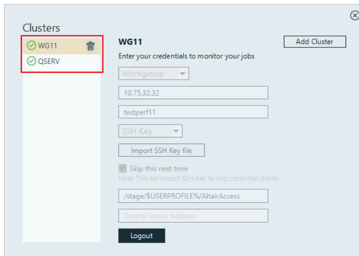
Figure 69: Clusters
