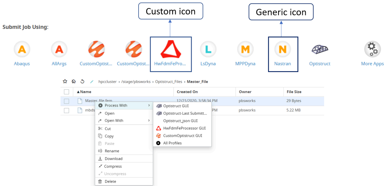
Figure 70: Application Icon in Job List and Context Menu
