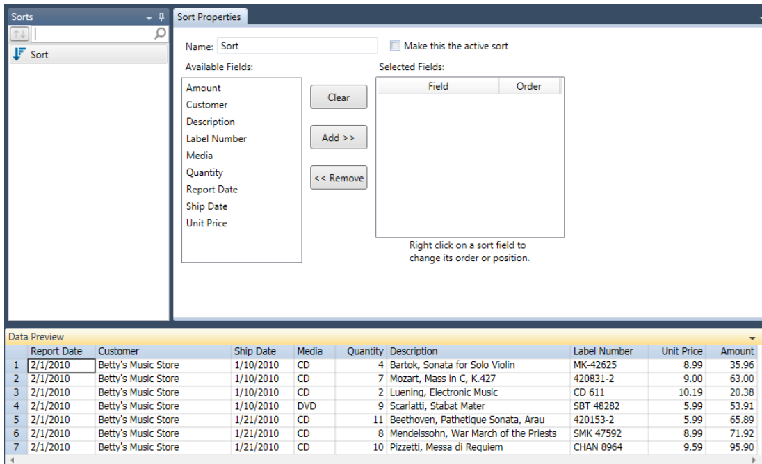
Figure 13-5. The Sort Order Definition window.
