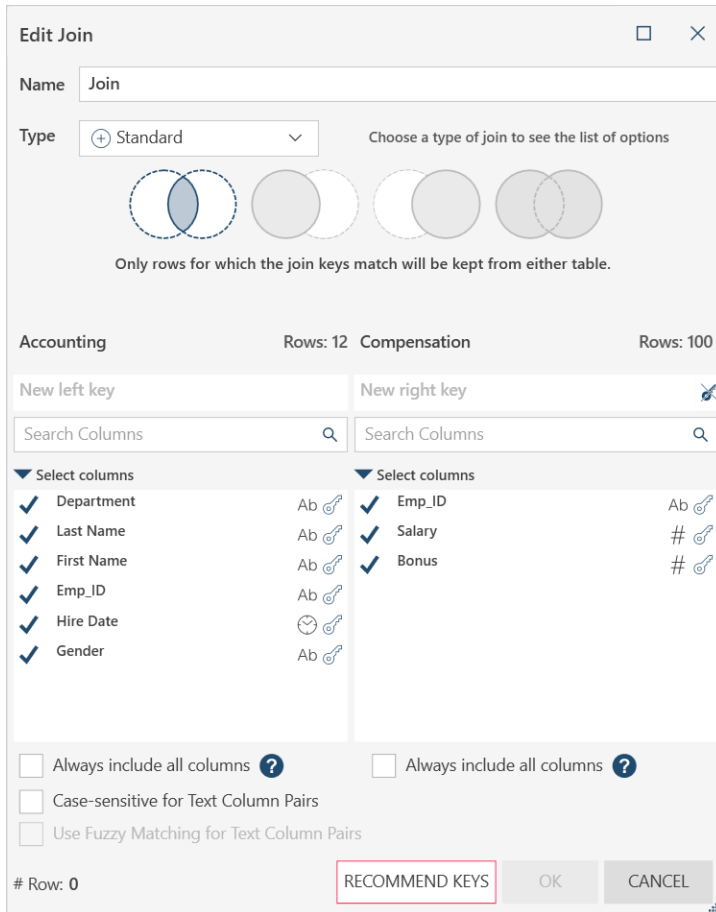
Figure 4-41. The resulting Join Configuration dialog.
