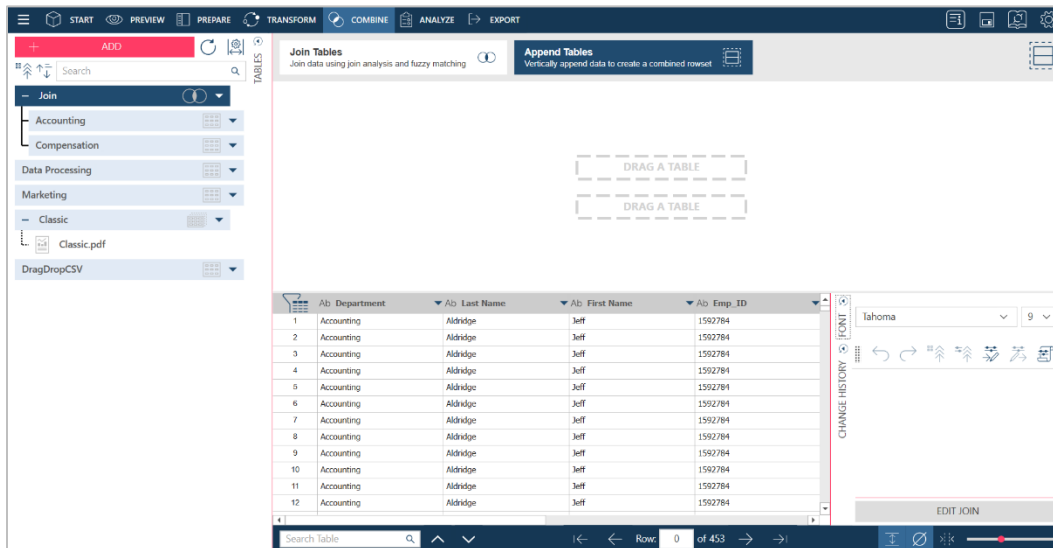
Figure 4-54. The Append stage.
