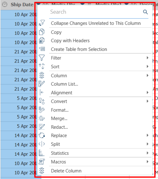
Figure 4-75. Available prep operations for Date/Time fields in the Prepare window.
