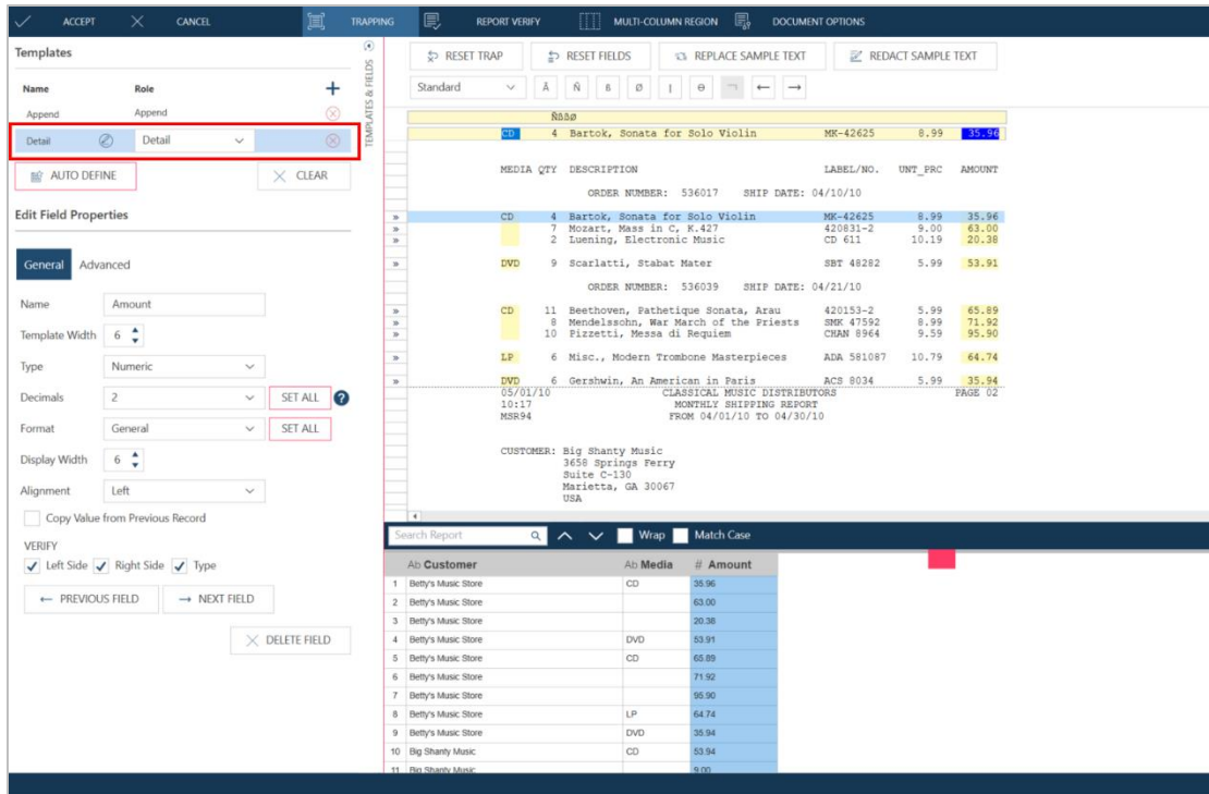
Figure 4-60. Extracting the Amount field from Classic.pdf via Report Design.
