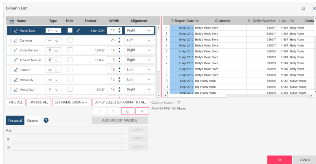
Figure 4-78. The Column List dialog.
