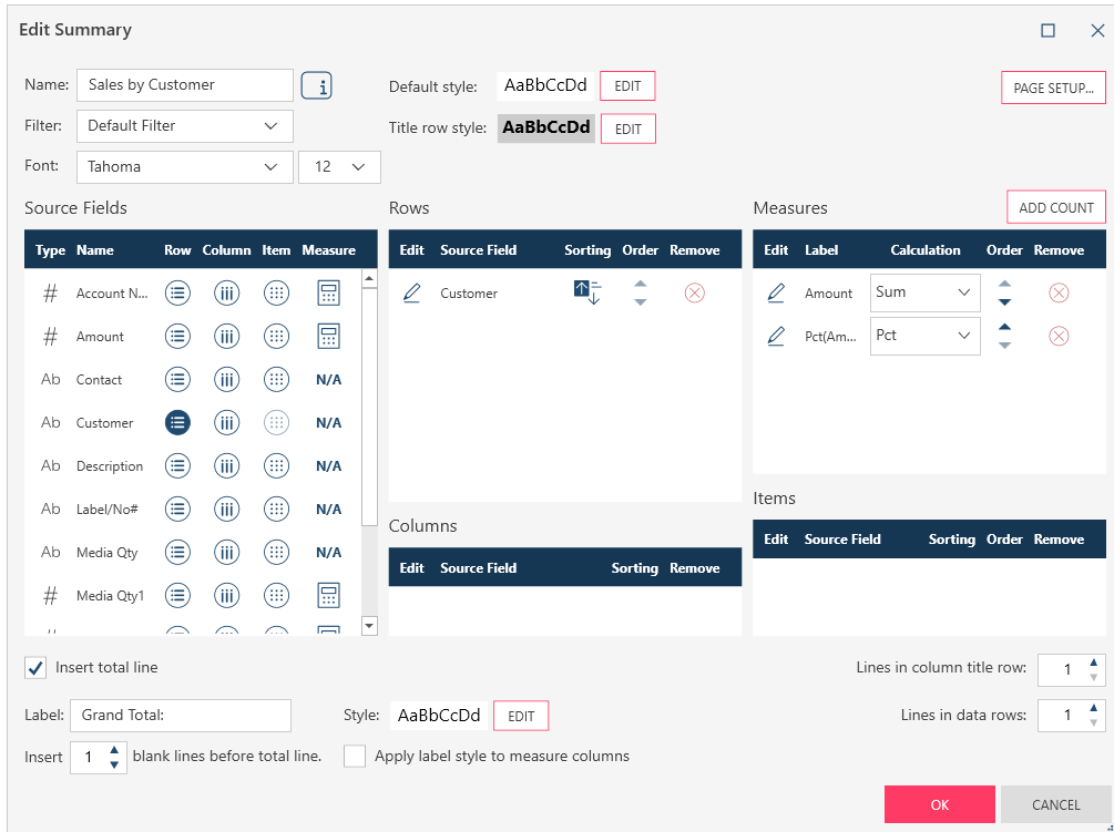
Figure 4-93. The Edit Summary dialog.
