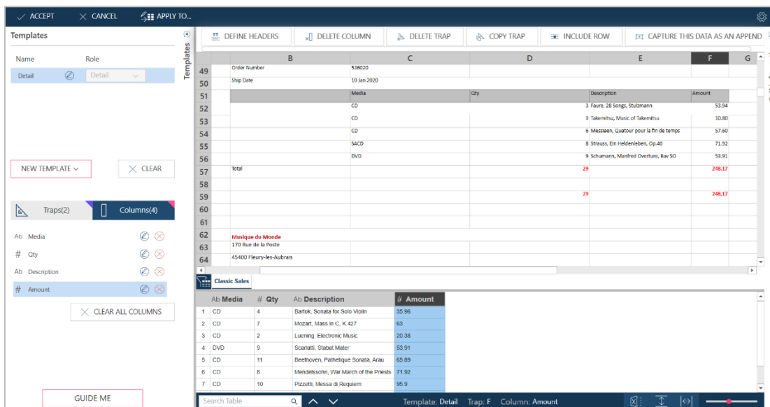
Figure 4-115. Checking for rows containing data that have not been captured correctly.
