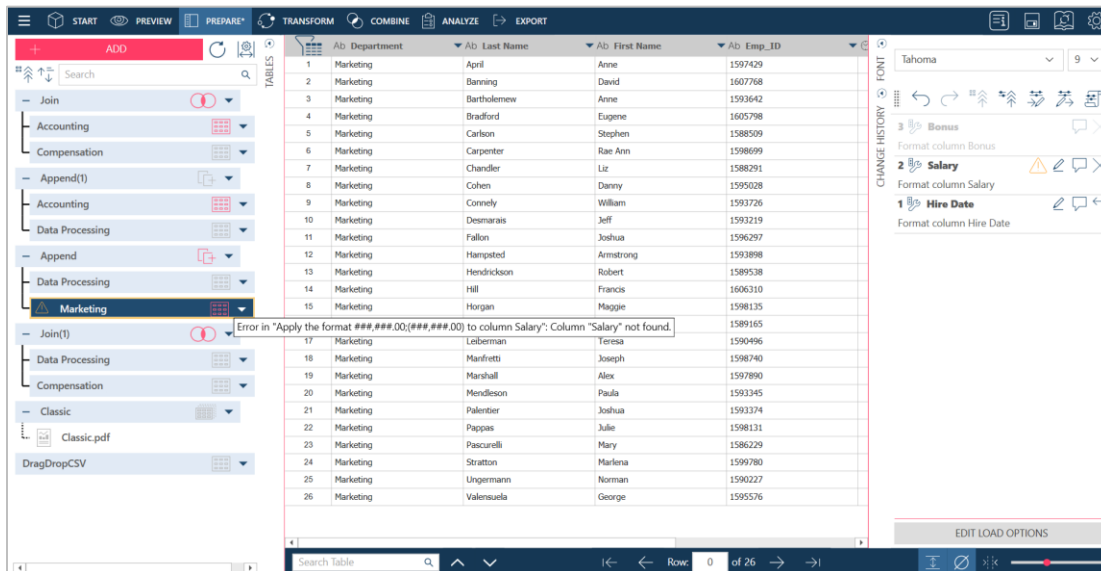
Figure 4-86. The change list created from the Join (Accounting + Compensation) table was dragged and dropped to the Marketing table.
