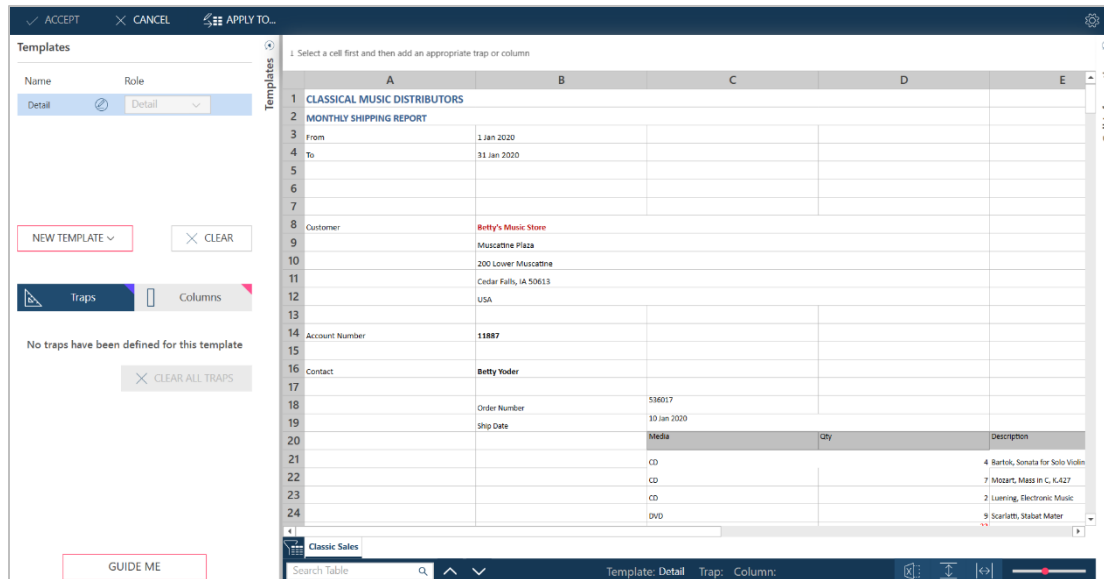
Figure 4-103. An open Excel report in Worksheet Design.
