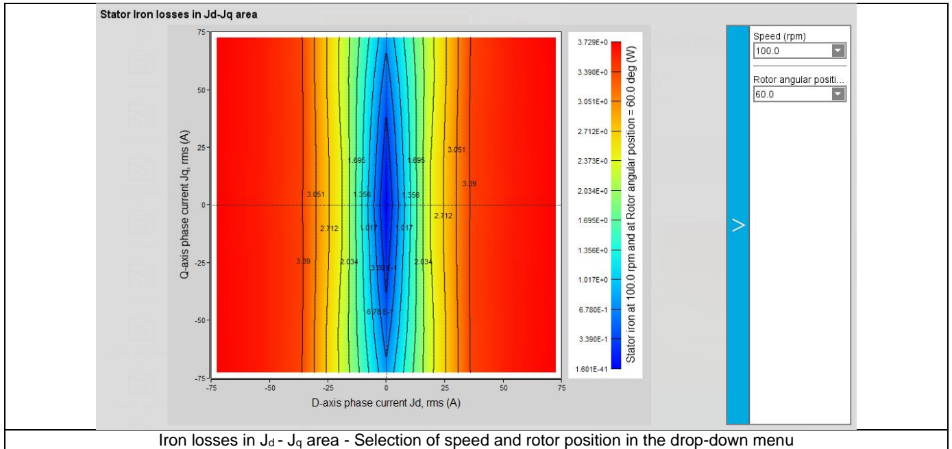
Iron losses in J_d - J_q area - Selection of speed and rotor position in the drop-down menu
