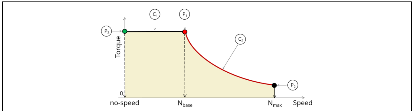
MTPV command modes – Torque-speed curve computation process
